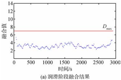
Fig. 12 Comparison of feature fusion value and effective value
