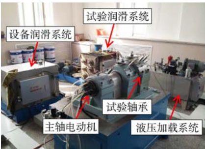
图 11 轴承失效监控系统 Fig. 11 Bearing failure monitoring system
