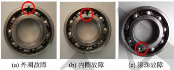
图 2 故障加工后的轴承 Fig.2 Bearings after fault processing
